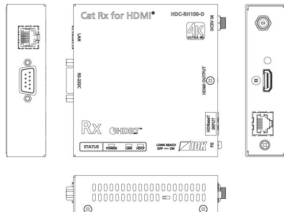
HDC-RH100-D
