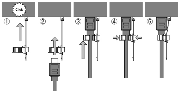
Securing HDMI cable using cable clamp
